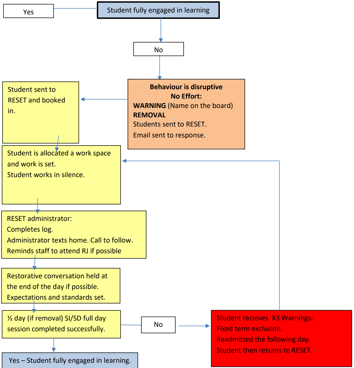
Referral Flowchart 1
